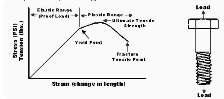
Figure 1 Tensile Stress-Strain Diagram
