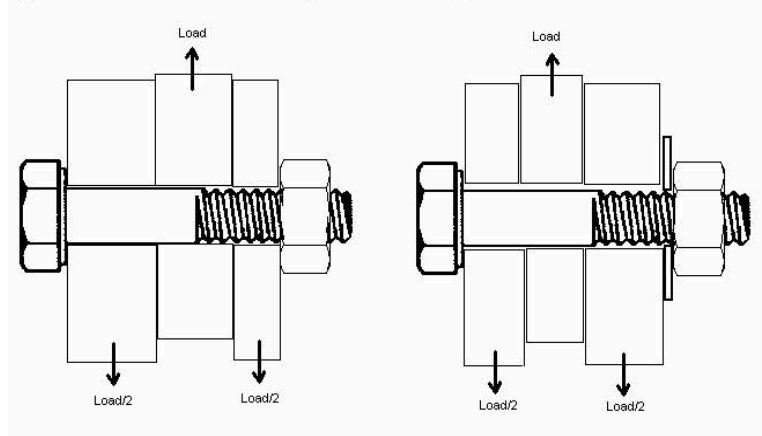
Figure 2 Shear Planes in a Bolted Joint
