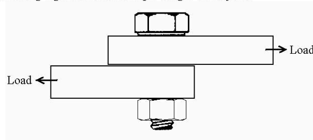
Shear Joint
